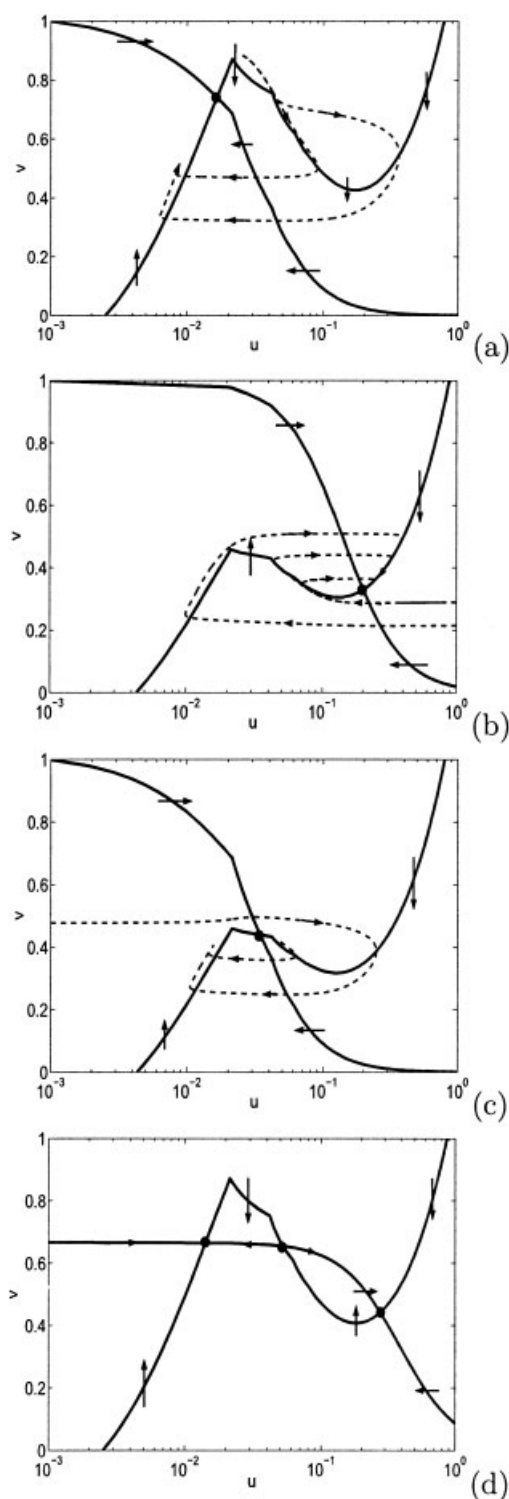
Figure 1. Phase-plane portraits of the system of Eq. 4, for different values of k'_2 , k''_2 , and k_{wee} .
