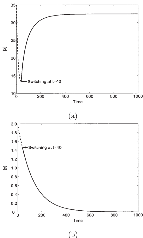
Figure 17. Time-evolution plots of the (a) CI and (b) Cro protein concentrations when the system initialized at [x(0), y(0)] = (35, 2) undergoes a transition from the \gamma_x = 0.05 mode (dashed lines) to the \gamma_x = 0.004 mode at t = 40 and converges (solid lines) to the lytic steady state.
