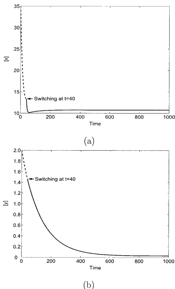
Figure 18. Time-evolution plots of the (a) CI and (b) Cro protein concentrations when the system initialized at [x(0), y(0)] = (35, 2) undergoes a transition from the \gamma_x = 0.05 mode (dashed lines) to the \gamma_x = 0.1 mode at t = 40 and converges (solid lines) to the lytic steady state.
