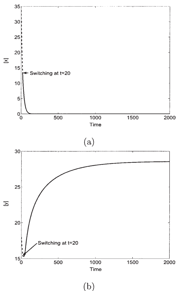
Figure 12. Time-evolution plots of the (a) CI and (b) Cro protein concentrations when the system initialized at [x(0), y(0)] = (35, 18) undergoes a transition from the \gamma_y = 0.008 mode (dashed lines) to the \gamma_y = 0.0005 mode at t = 20 and converges (solid lines) to the lytic steady state.
