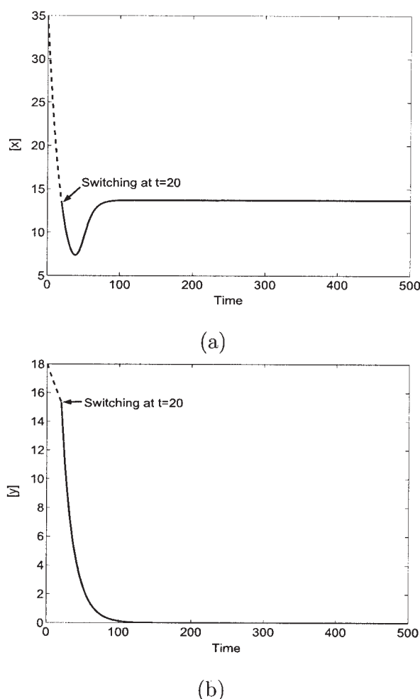
Figure 13. Time-evolution plots of the (a) CI and (b) Cro protein concentrations when the system initialized at [x(0), y(0)] = (35, 18) undergoes a transition from the \gamma_y = 0.008 mode (dashed lines) to the \gamma_y = 0.06 mode at t = 20 and converges (solid lines) to the lysogenic steady state.
