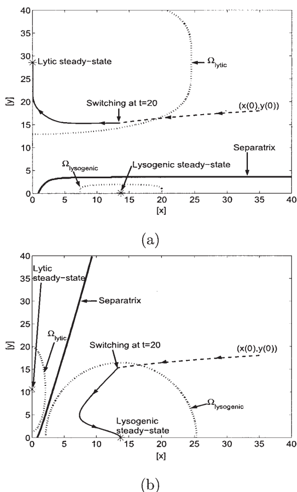
Figure 11. Phase plot showing the system of Eq. 5 being initialized using \gamma_y = 0.008 (dashed trajectory) and undergoing: (a) a decrease in the degradation rate of Cro protein (to \gamma_y = 0.0005 ) at t = 20 , leading the state to converge to the lytic steady state, and (b) an increase in the degradation rate of Cro protein (to \gamma_y = 0.06 ) at t = 20 , leading the state to converge to the lysogenic steady state.
